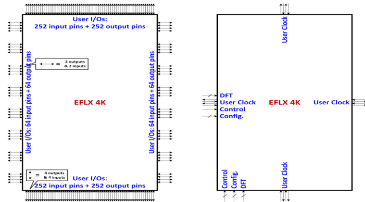
GF12 EFLX4K dimensions: 0.98 wide x 1.39mm tall
